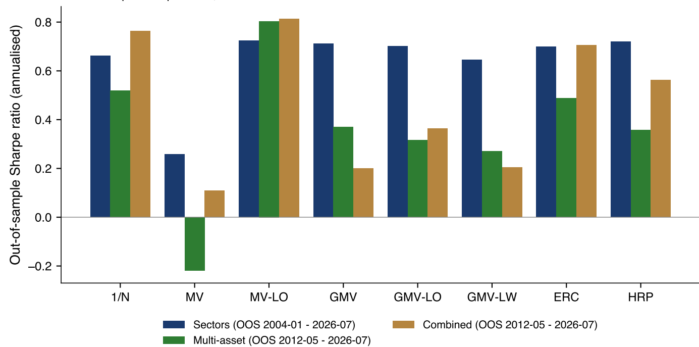
Out-of-sample Sharpe ratios, before costs
