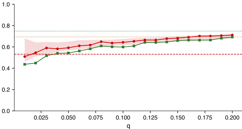
Tail dependence estimate
