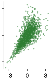
Clayton \theta = 2.00
