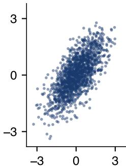
Gaussian \rho = 0.71
