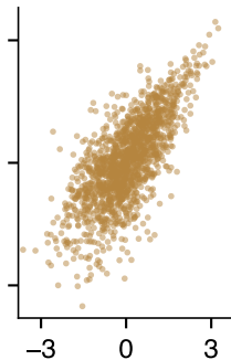
Gumbel \theta = 2.00
