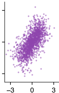
Frank \theta = 5.74
