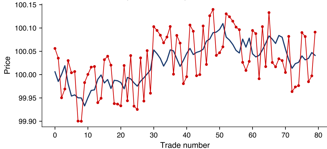
Simulated bid-ask bounce ( c = 0.05 , \sigma = 0.02 )
