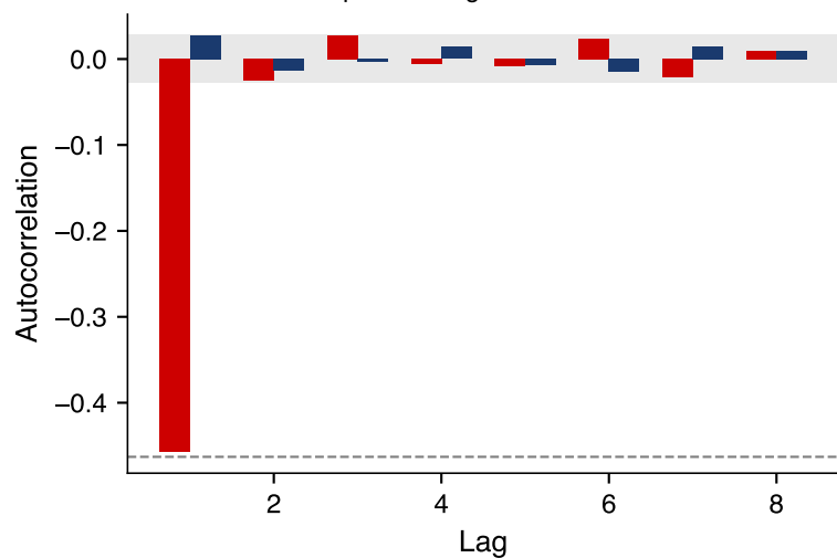
Autocorrelation of price changes
