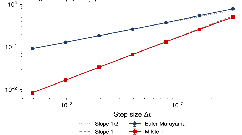
Strong error E|X_T - X_T^{\Delta t}|
