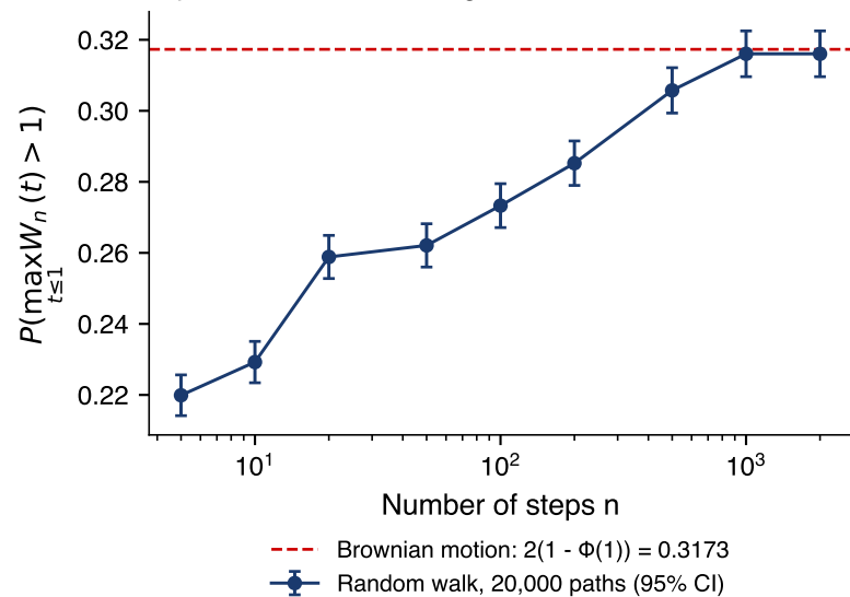
A path functional converges too
