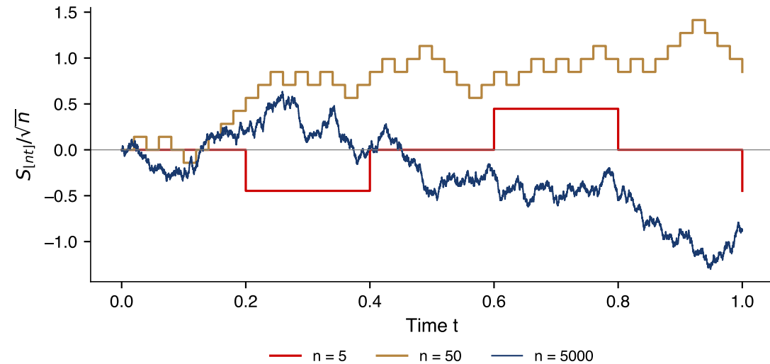
Scaled random walks
