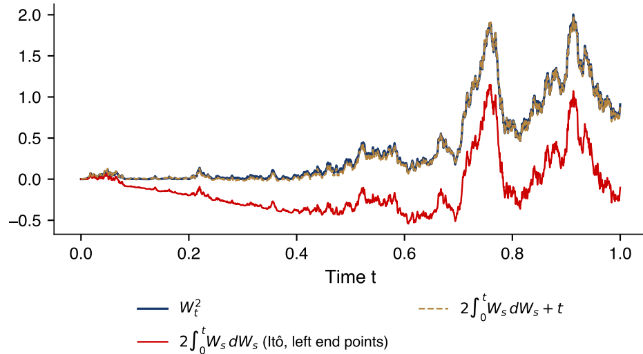
Itô's formula on one path
