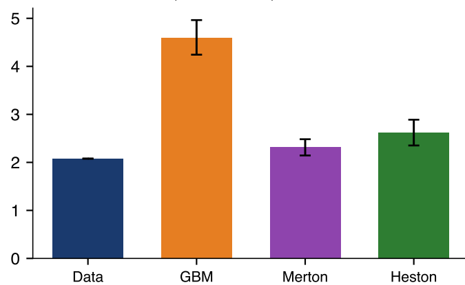
Bitcoin: Hill tail index (5% of losses)
