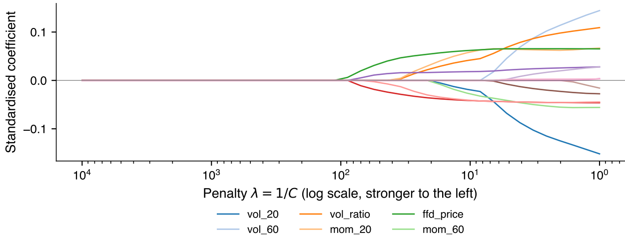
LASSO-logistic path, S&P 500 5-day direction: most features are shrunk to zero
