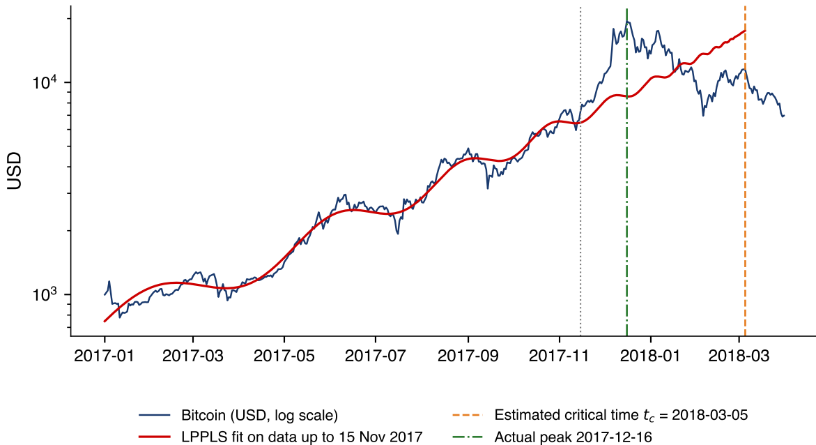
LPPLS on the 2017 Bitcoin bubble
