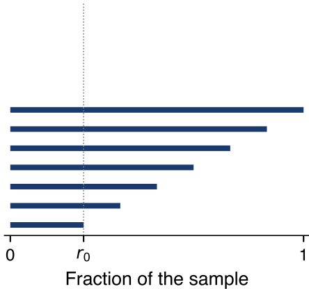
SADF: start fixed, end grows
