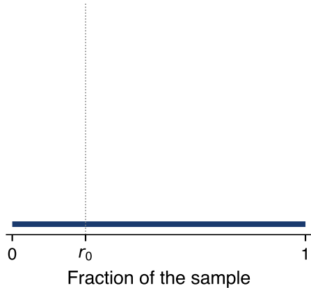
ADF: one window
