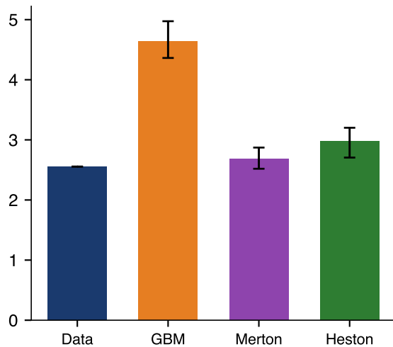
Hill tail index (5% of losses)
