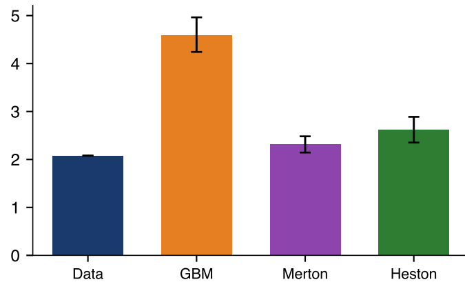
Bitcoin: Hill tail index (5% of losses)
