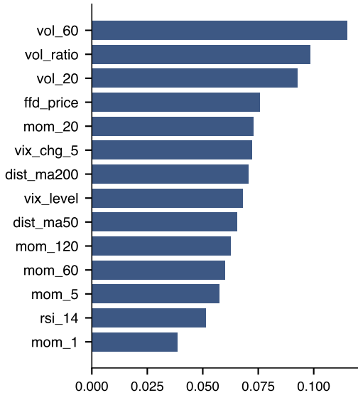
MDI (in-sample)
