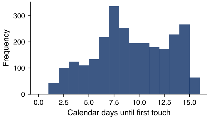
Horizontal barrier hits
