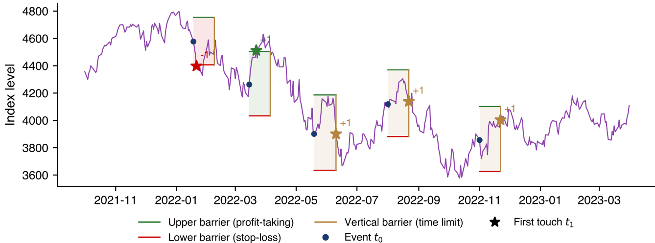
Triple-barrier labelling: barriers at \pm\sigma_{t_0}\sqrt{h} , h = 15 days
