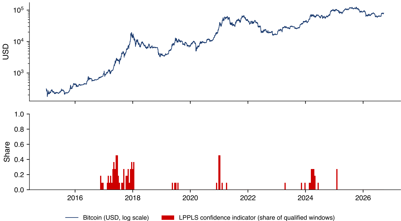
Bitcoin: real-time LPPLS confidence indicator, 11 windows of 90-690 days, every 2 weeks
