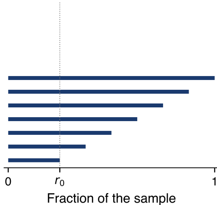
SADF: start fixed, end grows
