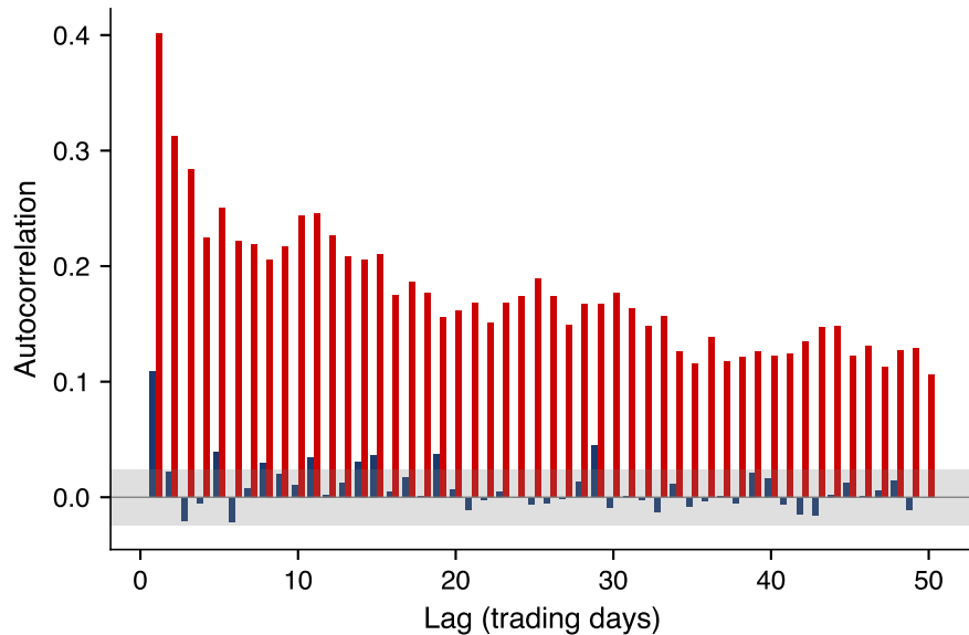
Autocorrelation function
