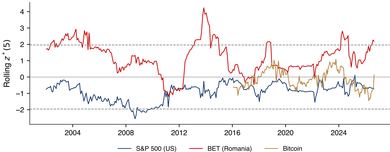
Time-varying efficiency: variance-ratio statistic on rolling 500-day windows
