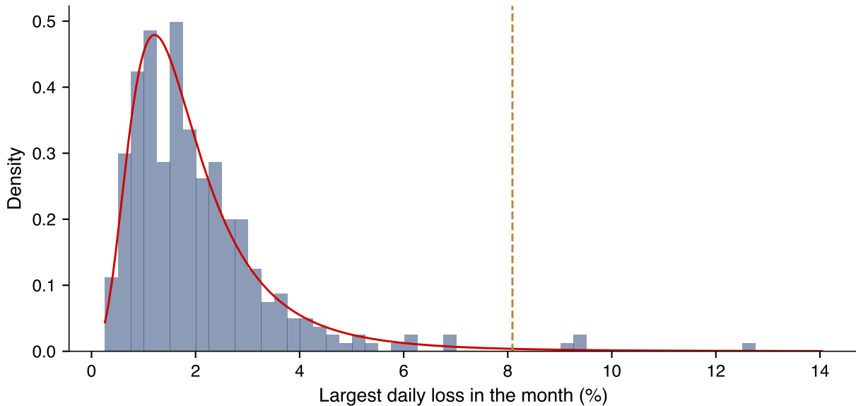
Block maxima: one maximum per calendar month, 2000-2026
