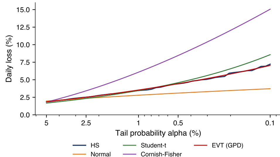
Value-at-Risk, S&amp;P 500 2000-2026
