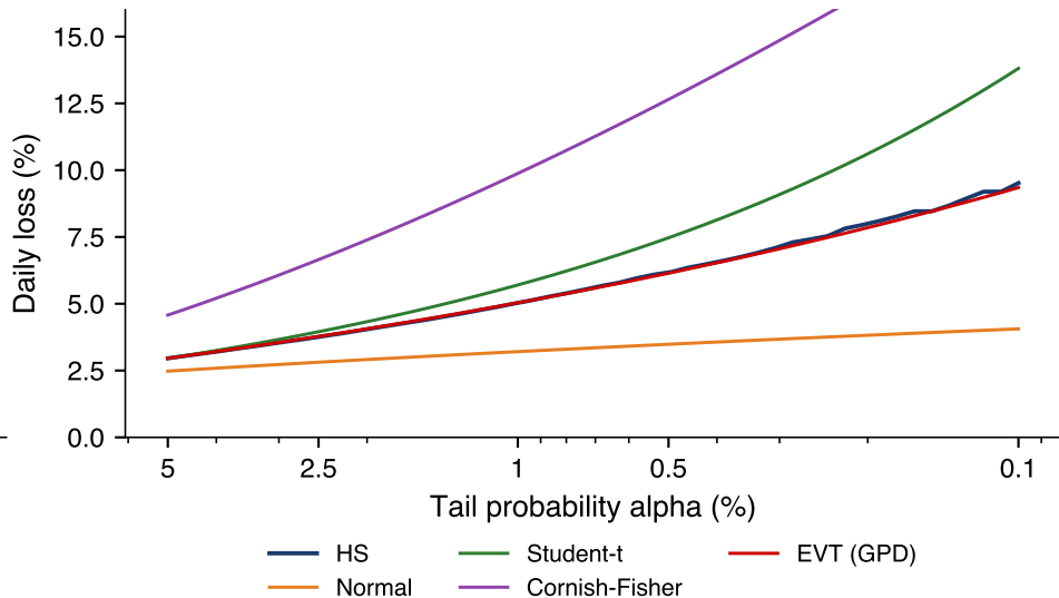
Expected Shortfall, S&amp;P 500 2000-2026
