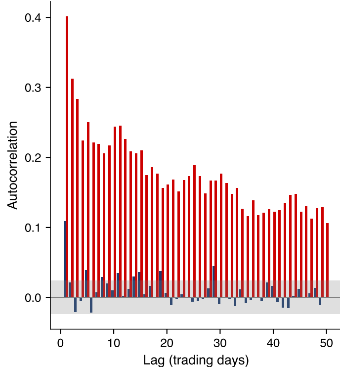
Autocorrelation function
