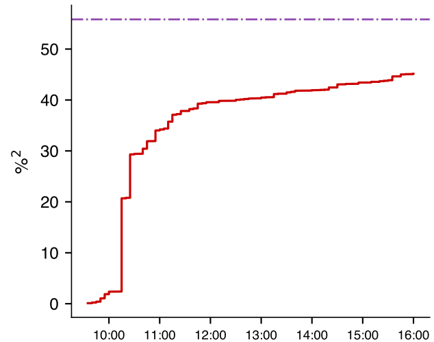
Realised variance
