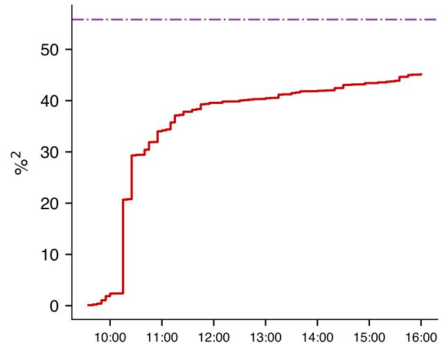
Realised variance
