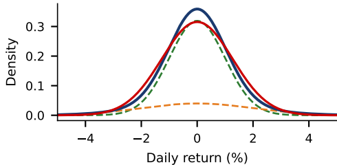
Higher peak than the Normal distribution
