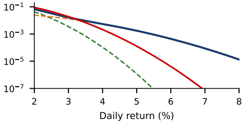
Right tail, log scale: heavier
