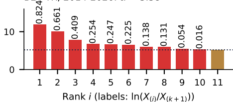
BET-TR, 2014-2026: \hat{\alpha} = 3.38
