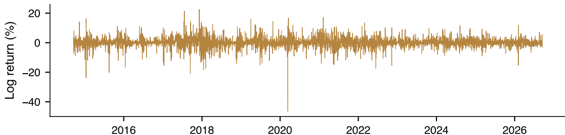
Bitcoin daily log returns, 2014-2026
