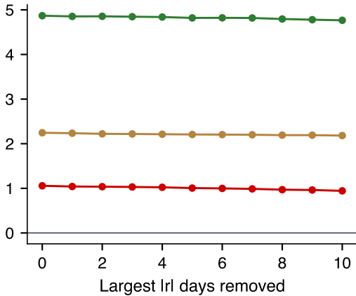
Crow-Siddiqui quantile kurtosis
