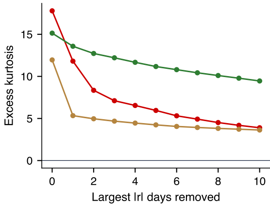
Moment excess kurtosis
