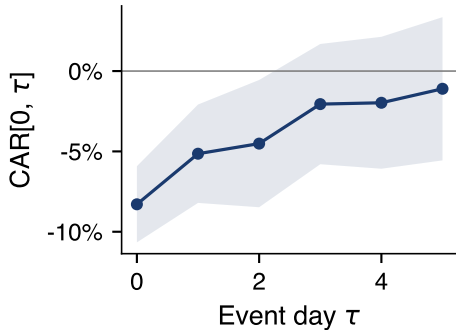
CAR with \pm 1.96 SE bands
