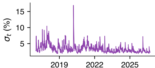
Conditional volatility
