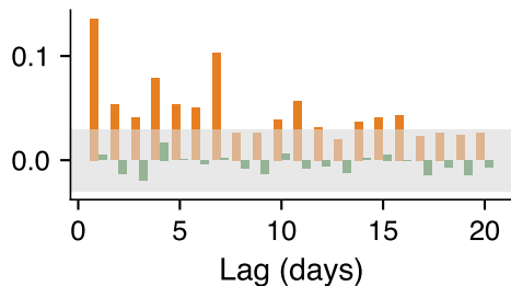
Clustering removed?
