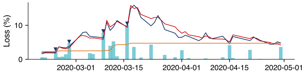
COVID-19 window, 20 Feb - 30 Apr 2020
