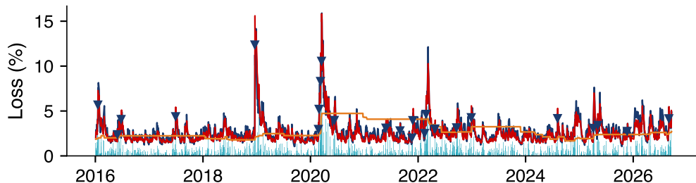
BET, 2016-2026: one-day-ahead VaR 1% out of sample
