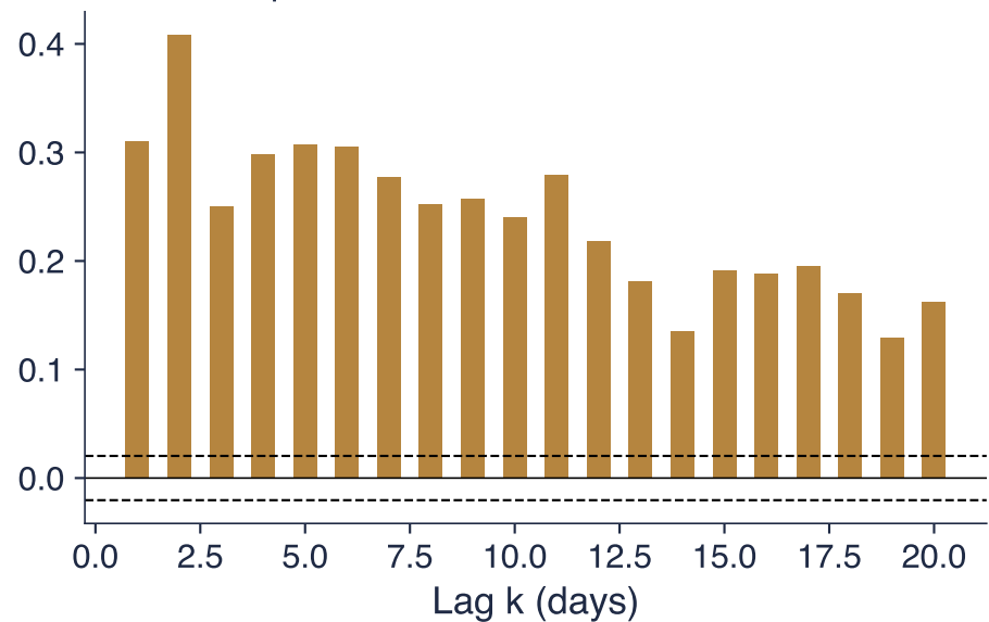
S&amp;P 500: squared returns
