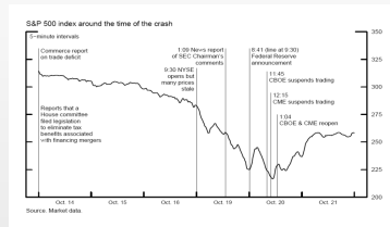
The S&P 500 around the crash of October 1987
