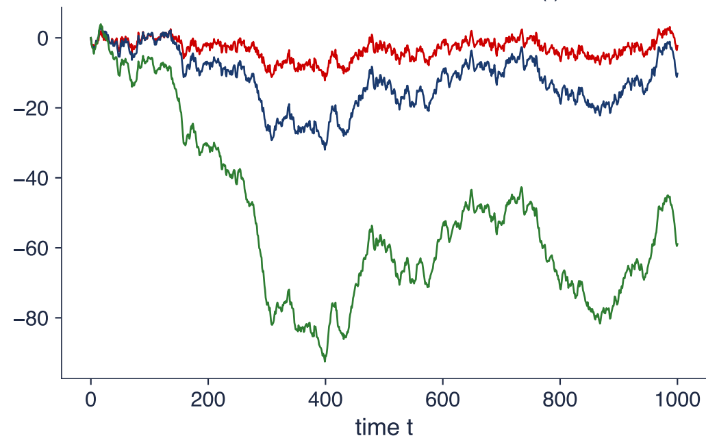
fractional Brownian motion B_H(t)
