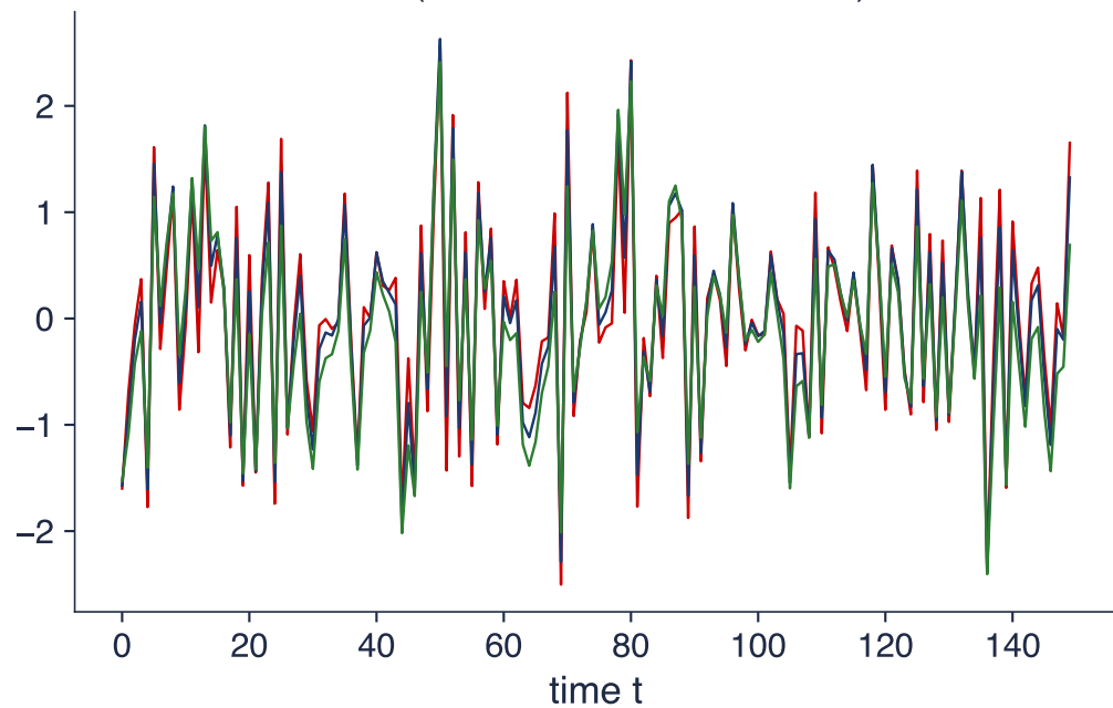
its increments (fractional Gaussian noise), first 150
