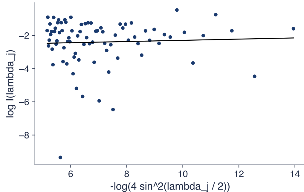
returns r: slope d = 0.04 (SE 0.07)
