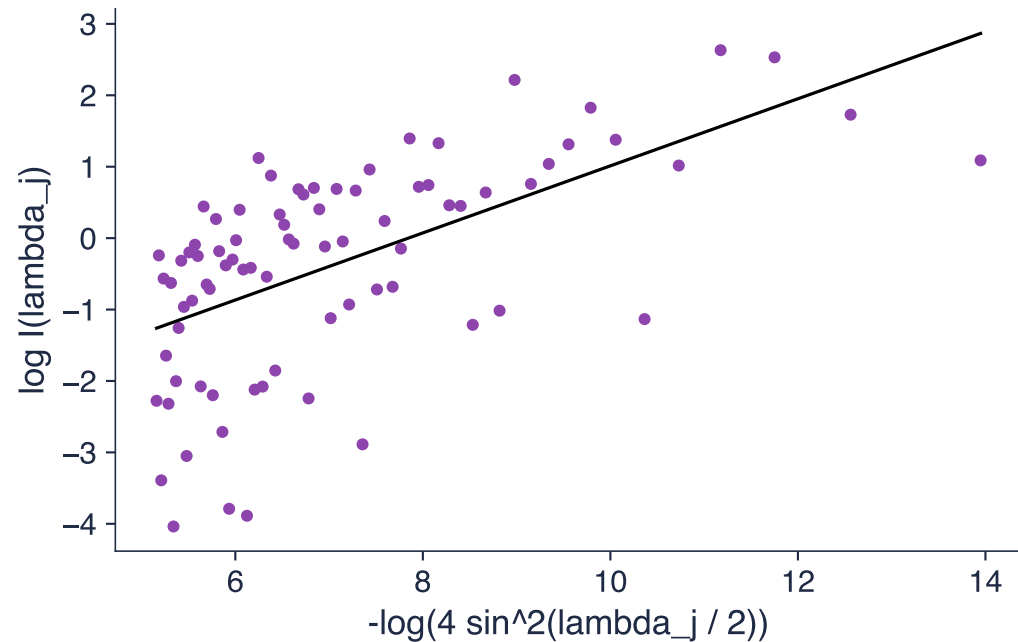
absolute returns lrl: slope d = 0.47 (SE 0.07)
