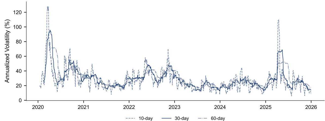
Historical Volatility: Window Sensitivity (AAPL)
