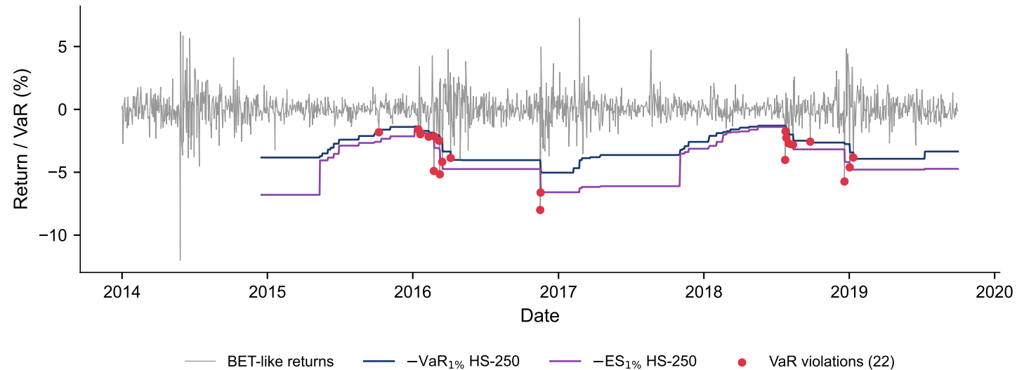
BVB case: rolling 250-day VaR/ES at 1% with crisis jump
