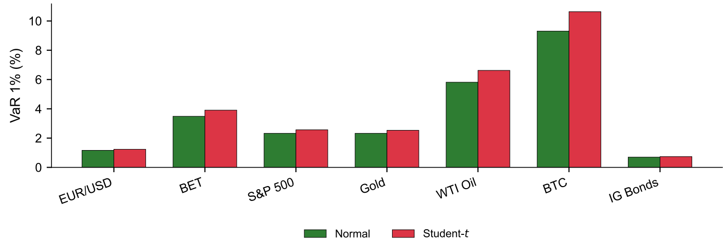
Cross-asset 1-day VaR 1\%: Normal vs Student- t
