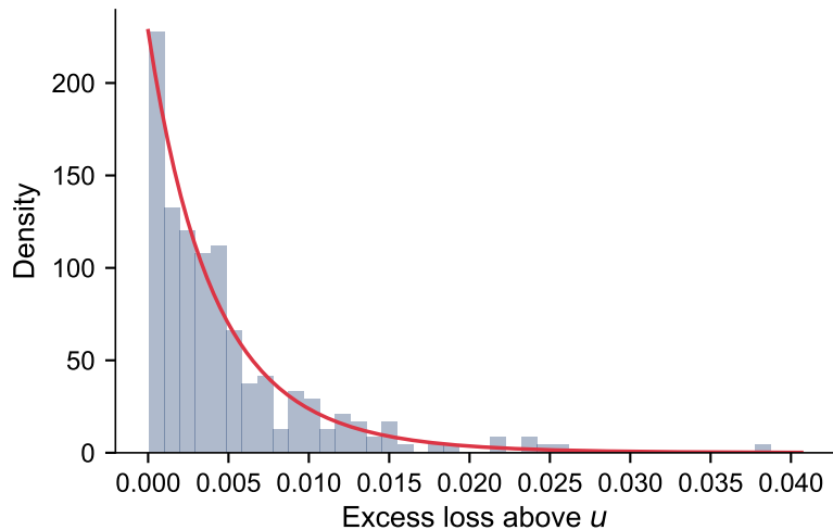
GPD fit to 250 excesses ( u=0.73\% )
