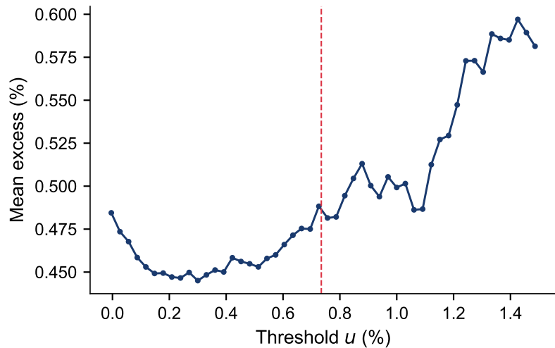
Mean-excess plot: linear \Rightarrow GPD tail
