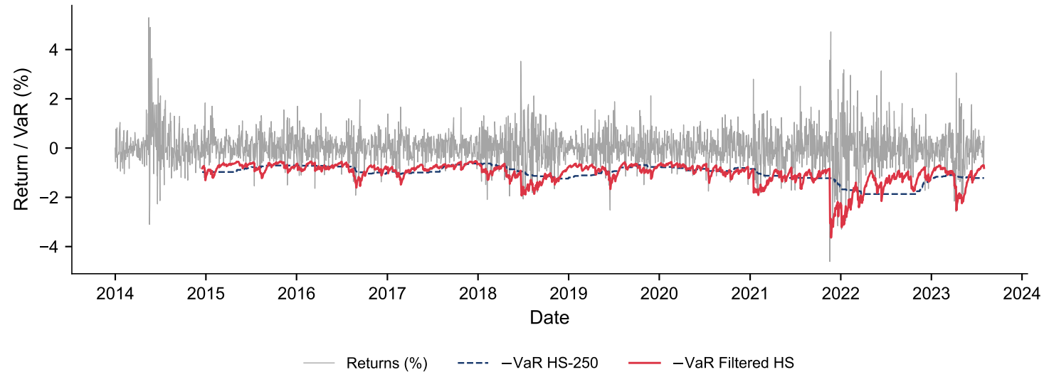
Filtered Historical Simulation: HS on z_t = (r_t - \mu)/\sigma_t
