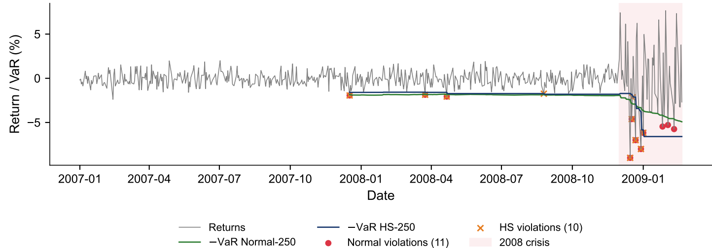
Lehman-style crisis: Normal-VaR fails, HS-VaR also struggles
