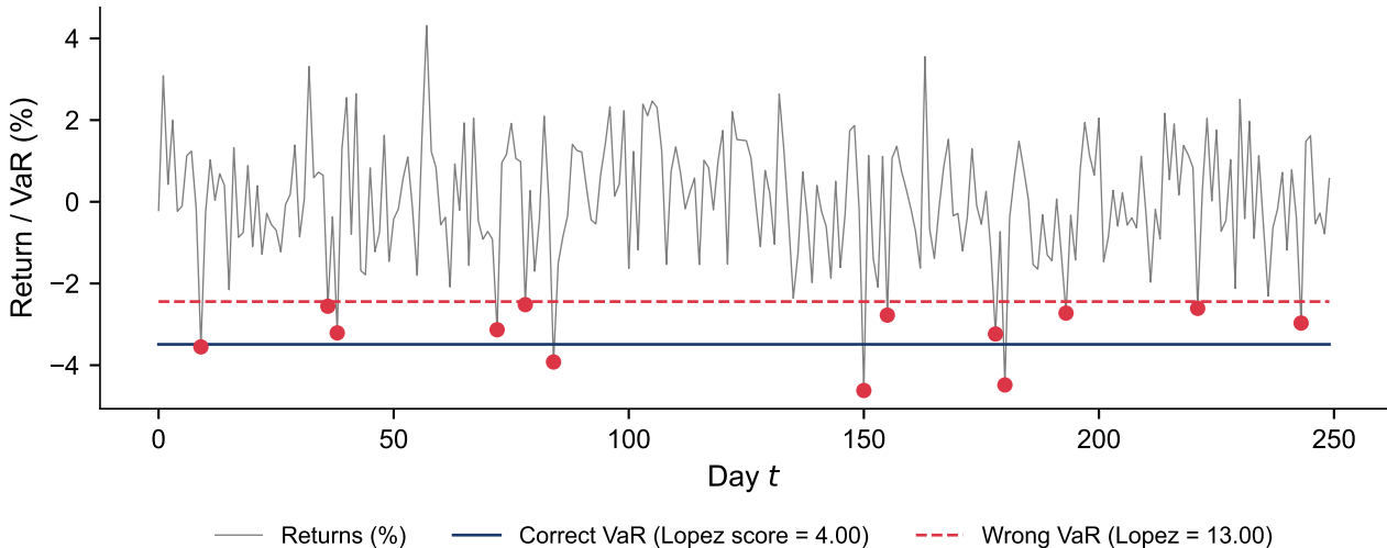
Lopez loss function: penalises magnitude beyond VaR
