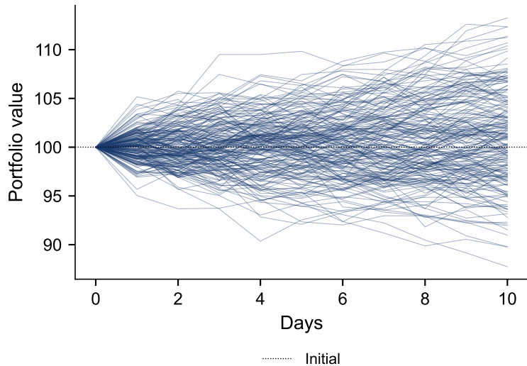
200 Monte Carlo paths (10-day horizon)
