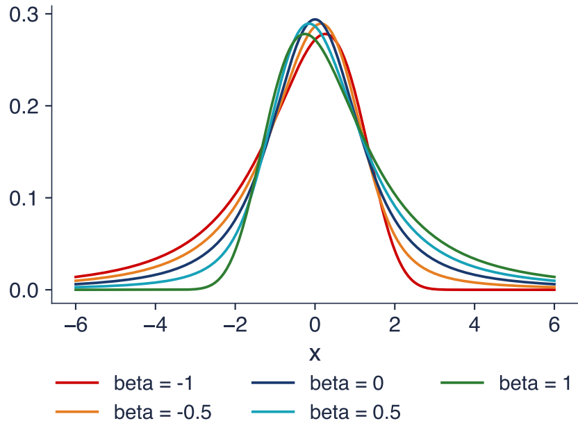
alpha = 1.3, gamma = 1: the effect of beta
