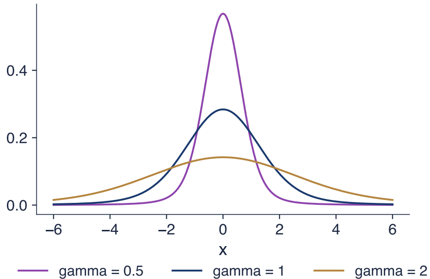
alpha = 1.7, beta = 0: the effect of gamma
