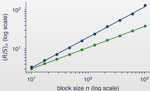
R/S regression, N = 4096 simulated returns
