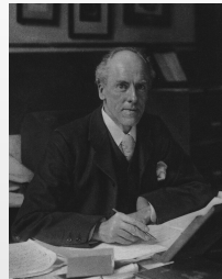
Karl Pearson (1857–1936)
