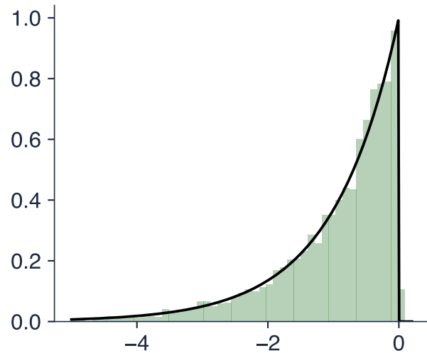
Uniform(0, 1): n(M - 1)
