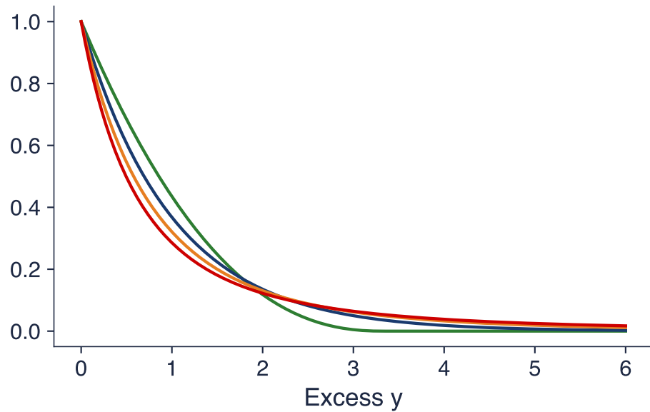
Density g(y)
