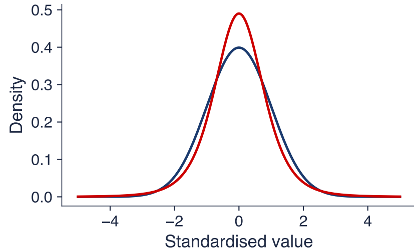
Kurtosis: taller centre, heavier tails
