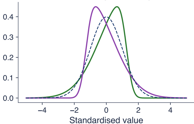
Skewness: a longer left or right tail
